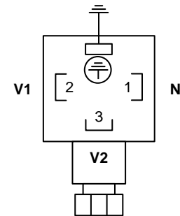
Fig. 7. Three pin electrical plug connector (according to ISO 4400) for IP applications.
