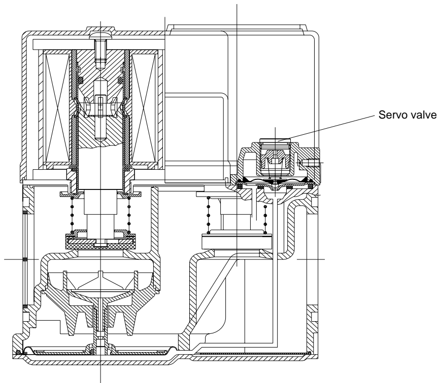
Fig. 17. Servo pressure regulator working
