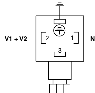
Fig. 8. Three pin electrical plug connector (according to ISO 4400) for DBI applications.
