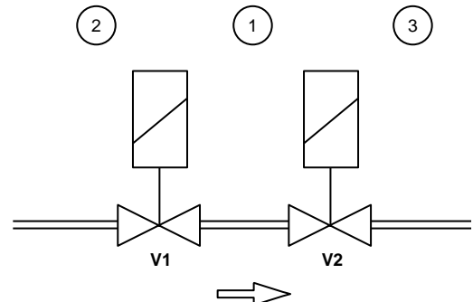
Fig. 9. Connection diagram VR400
