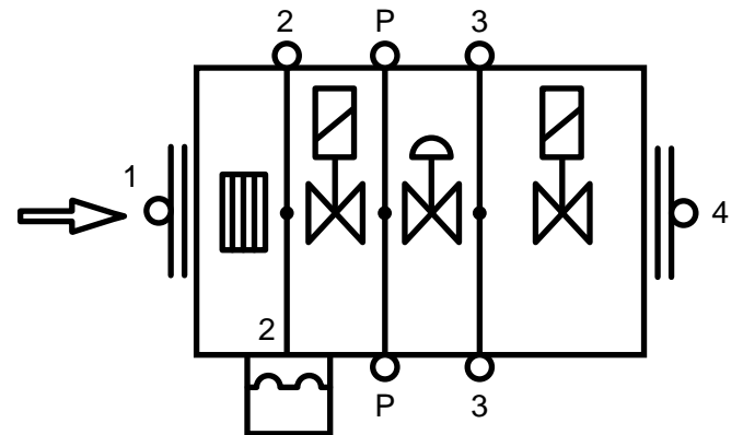
Fig. 16. Pressure tap points
