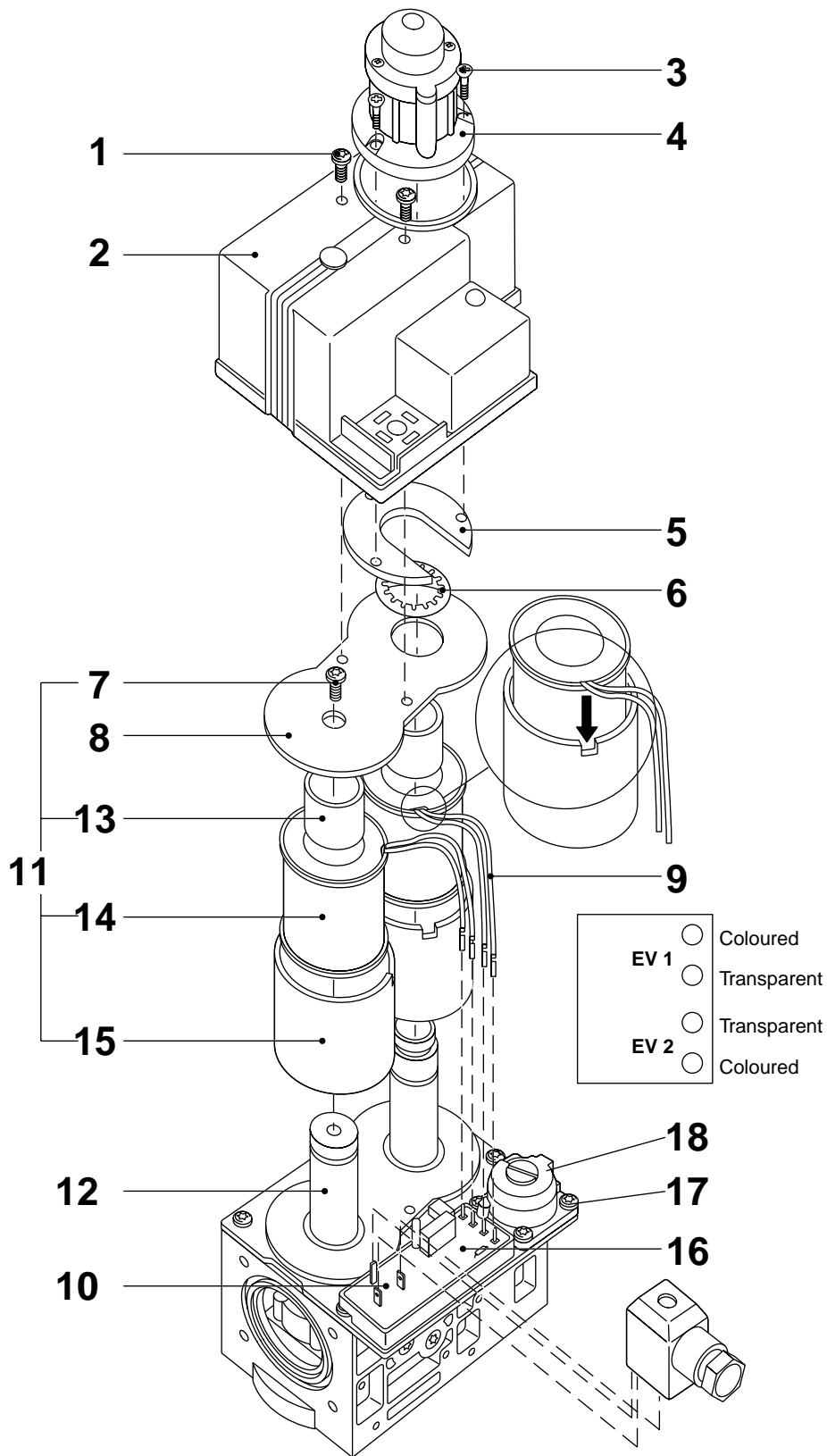
Fig. 19. Exploded view of the VR400/VR800 series
