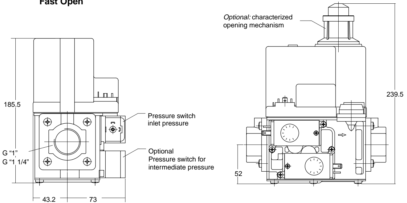
Fig. 6. Dimensional drawing VR425/VR825 series (DN25) and VR432/VR832 series (DN32)
